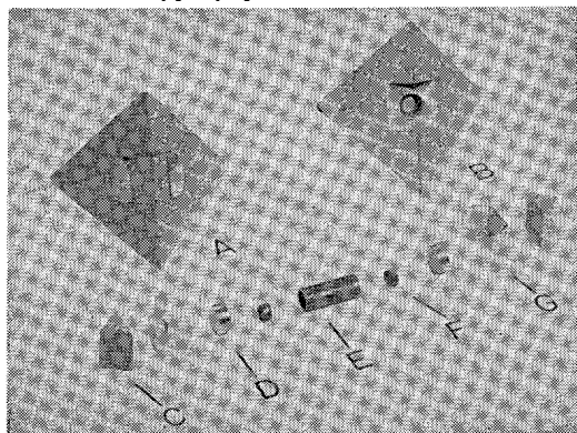
FIG. 1. Pyrophyllite sample-holder and assembly.
