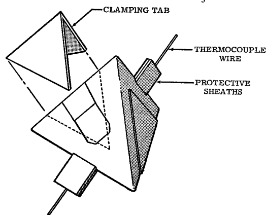
FIG. 3. Assembled sample, showing protective sheaths for thermocouple.
