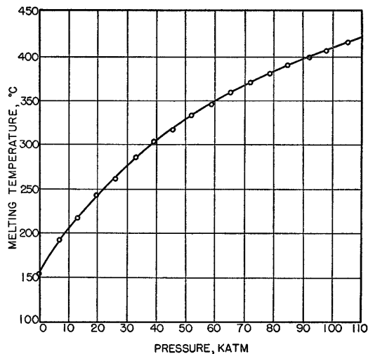
FIG. 6. Fusion curve of indium.
