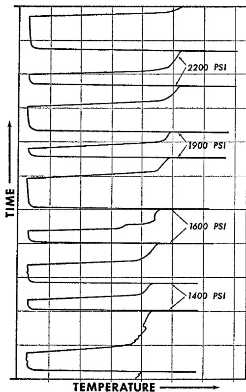
FIG. 5. Typical strip-chart record of melting.
