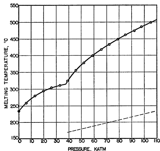
FIG. 7. Fusion curve of tin.
